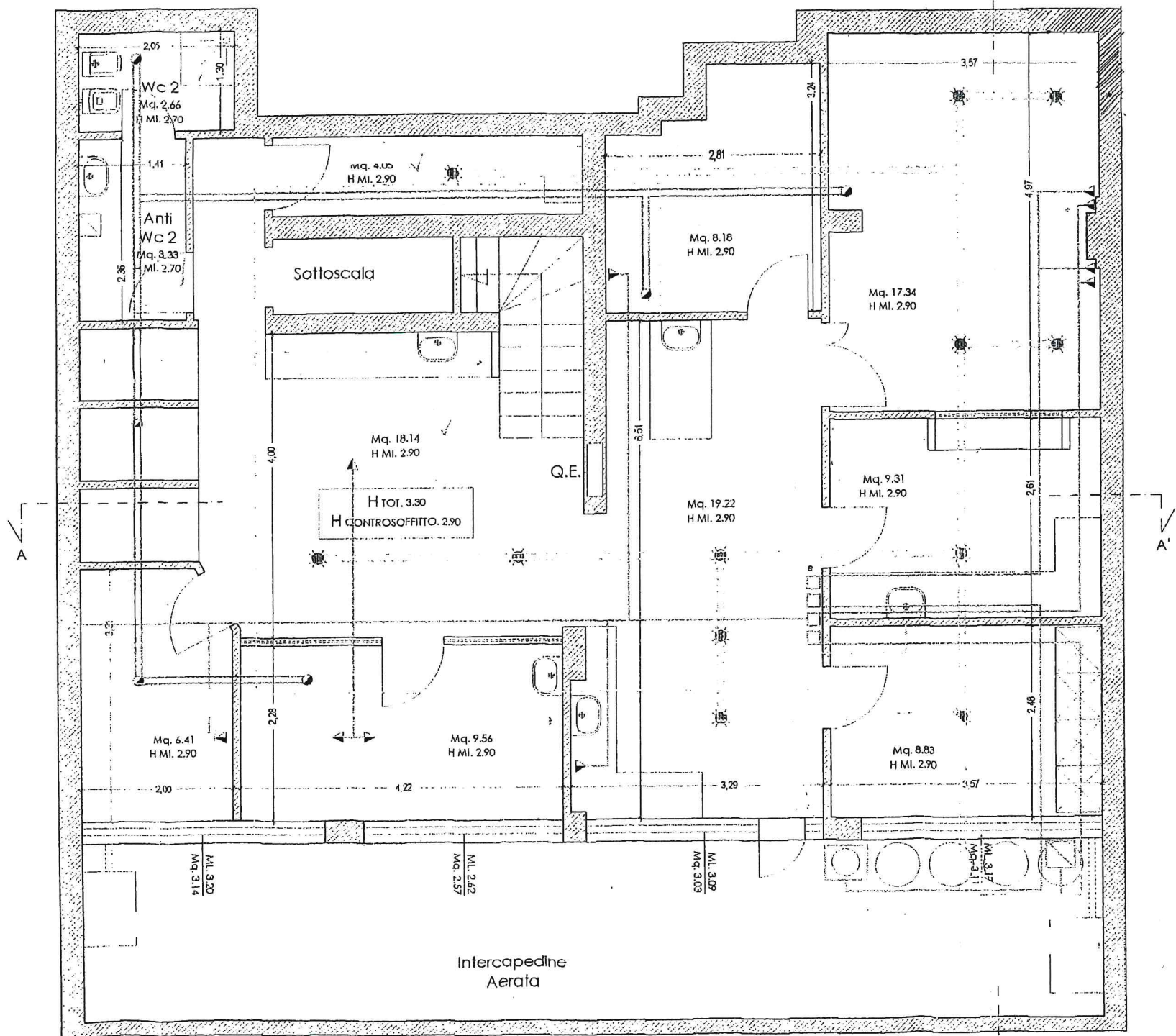
PIANO SEMINTERRATO Scala 1:50
